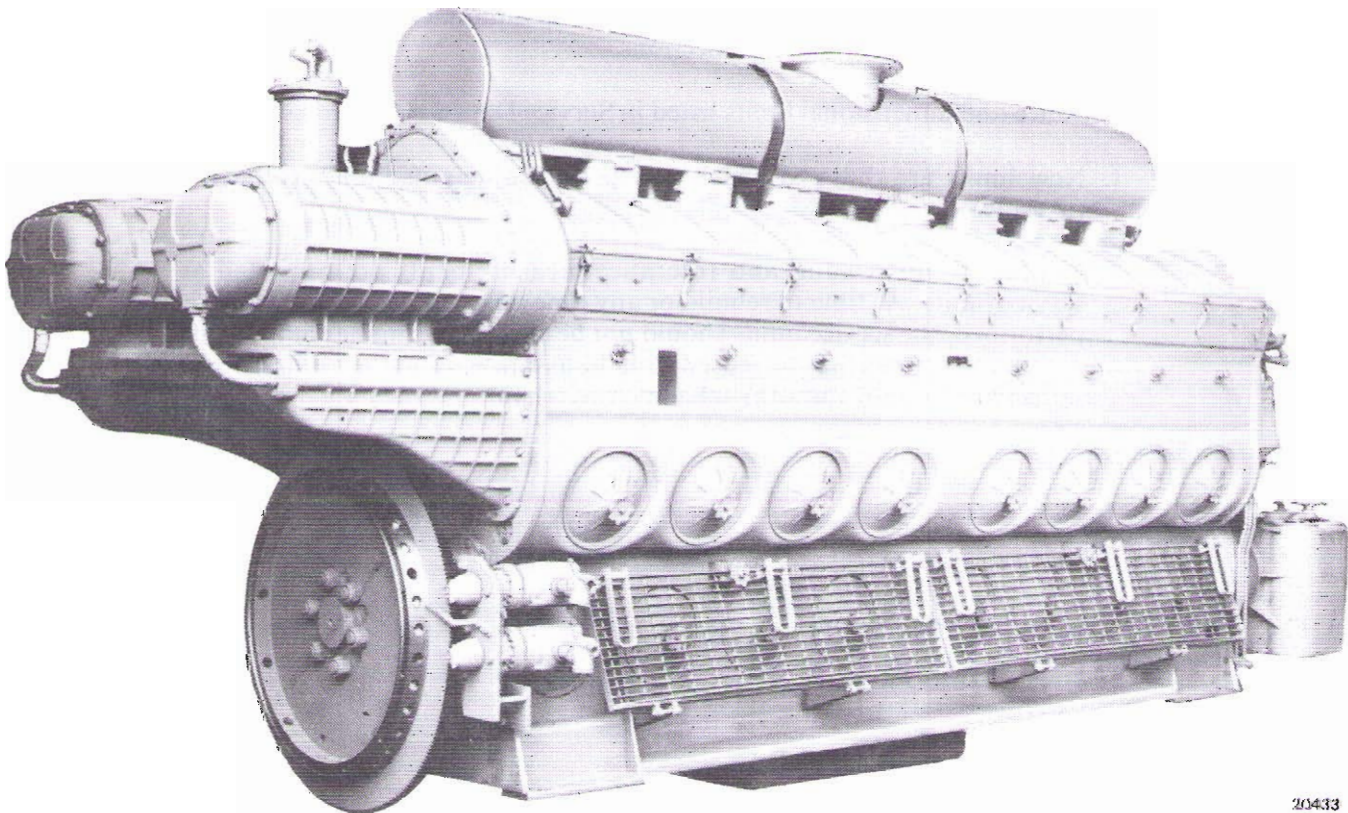
Three-Quarter Right Rear View, 16-Cylinder Engine
