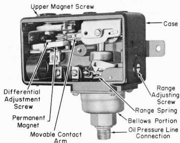
Fig. 3 - Low Oil Pressure Adjustment
