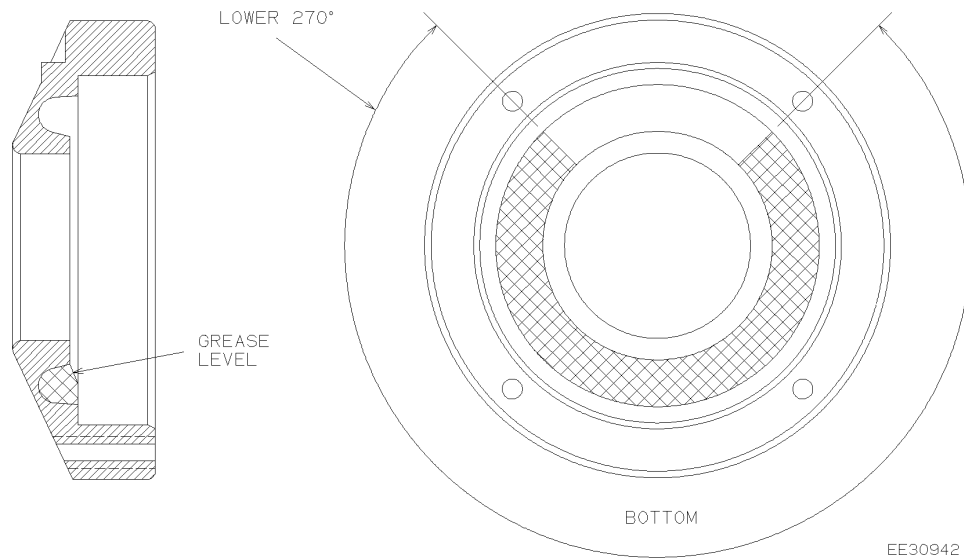
Fig. 10 - End Frame and Bearing Housing Grease
