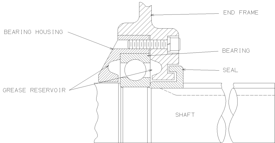
Fig. 11 - Bearing Assembly, Cross-Section
