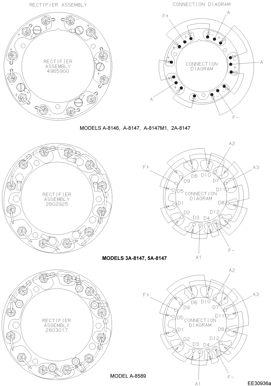
Fig. 5 - Rectifier Assembly Configurations
