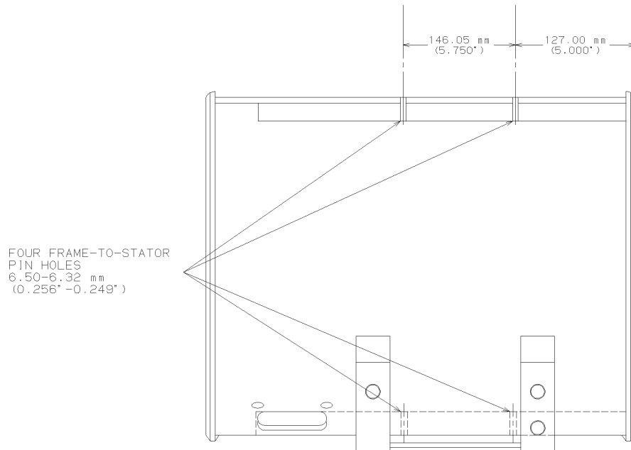
Fig. 8 - Frame-to-Stator-Pin Holes Location
