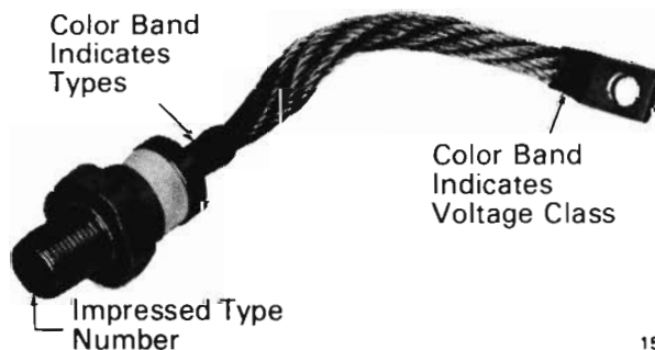
Fig.12 - Diode Type-Number And Color Bands
