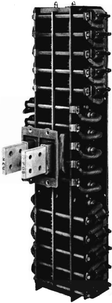
Fig.1 - Fabricated-Type Rectifier Bank Assembly
