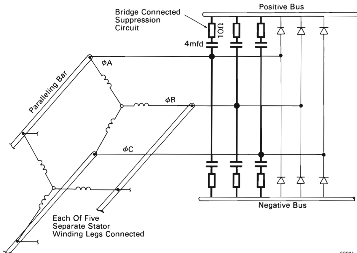
Fig.15 – Bridge Connected Suppression Circuit, Simplified Diagram
