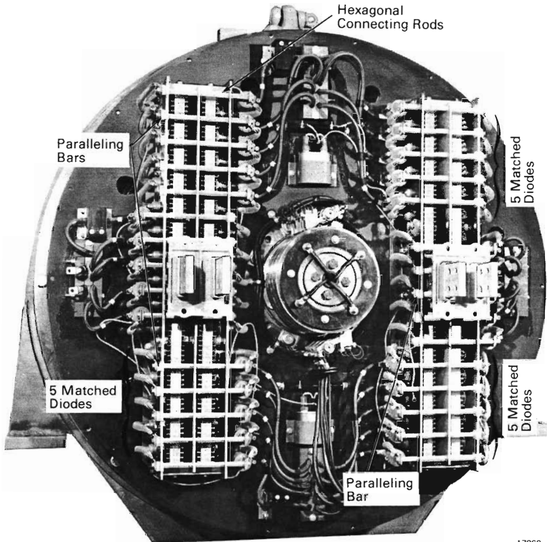
Fig.14 - Diode Matching Within Groups
